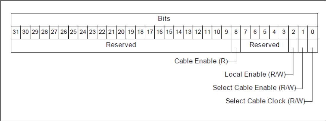
図B-18 RCIM III POSIX Clock Skip/Add Time Register
