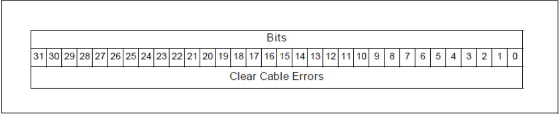
図A-15 RCIM IV Output Cable Status Register
