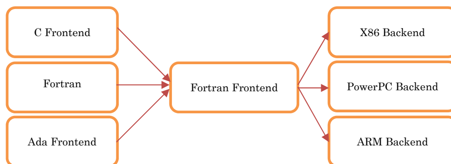
The LLVM Compilation Framework
